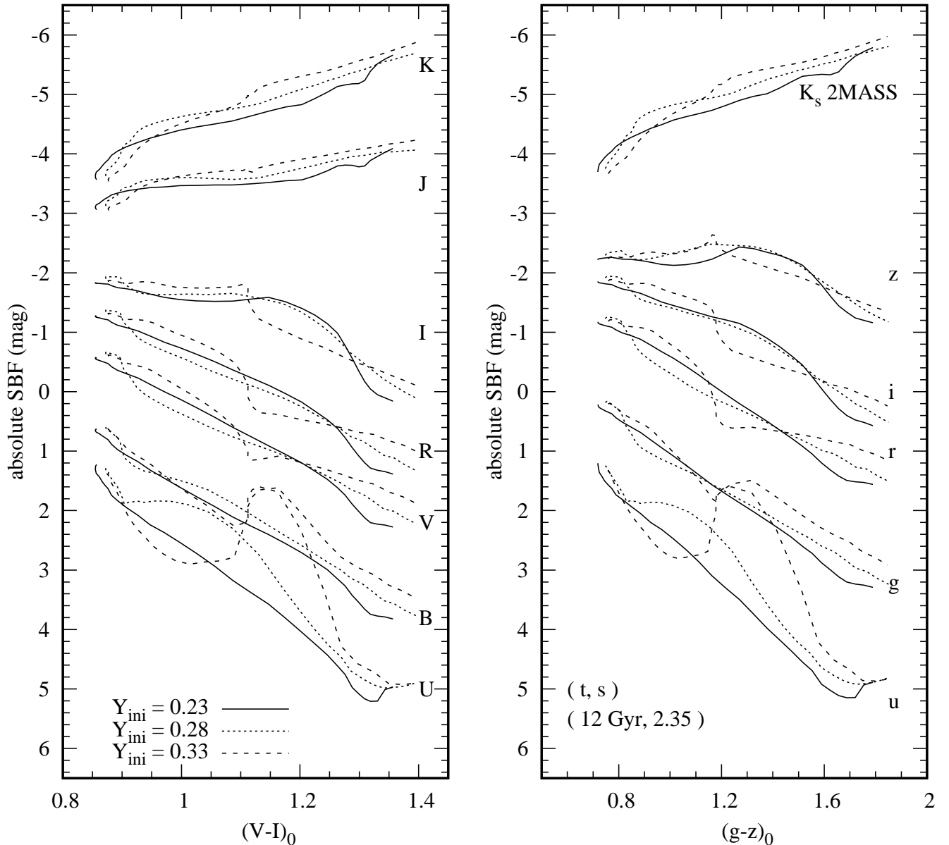
Figure 5. YEPS models in the SBF versus integrated color planes with different assumptions on the initial He. ( Left panel ) The same as Figure 4 but for the (V - I)_0 color. ( Right panel ) SDSS ugriz and 2MASS K_s SBFs as functions of the (g - z)_0 color. All SBF magnitudes are given in the Vega mag system. The (V - I)_0 color is based on the Vega mag system, while the (g - z)_0 color is in the AB mag system. The model parameters used for the comparison are denoted in the parenthesis in the right panel.
