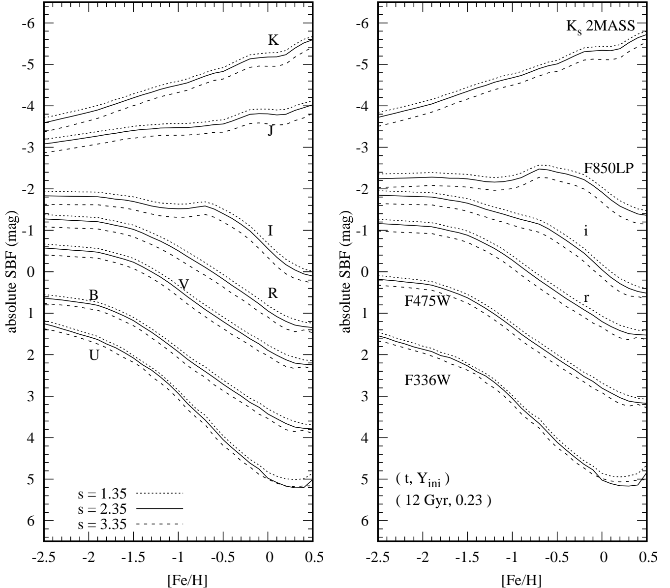
Figure 6. Same as Figure 3, but for the effect of the slope of the IMF on the SBF amplitudes. The dotted, solid, and dashed lines are, respectively, for the adopted Salpeter indices of s = 1.35 , 2.35 , and 3.35 . The model parameters used for the comparison are denoted in the parenthesis in the right panel.
