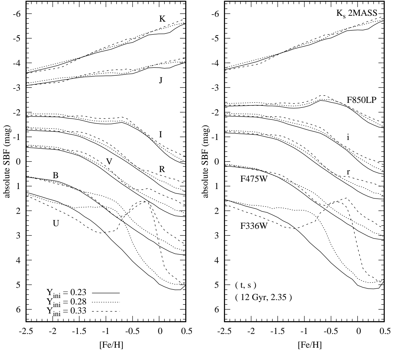
Figure 4. Same as Figure 3, but for the effect of initial He on the SBF amplitudes. The solid, dotted, and dashed lines are, respectively, for the SBF models for Y_{\text{ini}} = 0.23 , 0.28 , and 0.33 . The model parameters used for the comparison are denoted in the parenthesis in the right panel.
