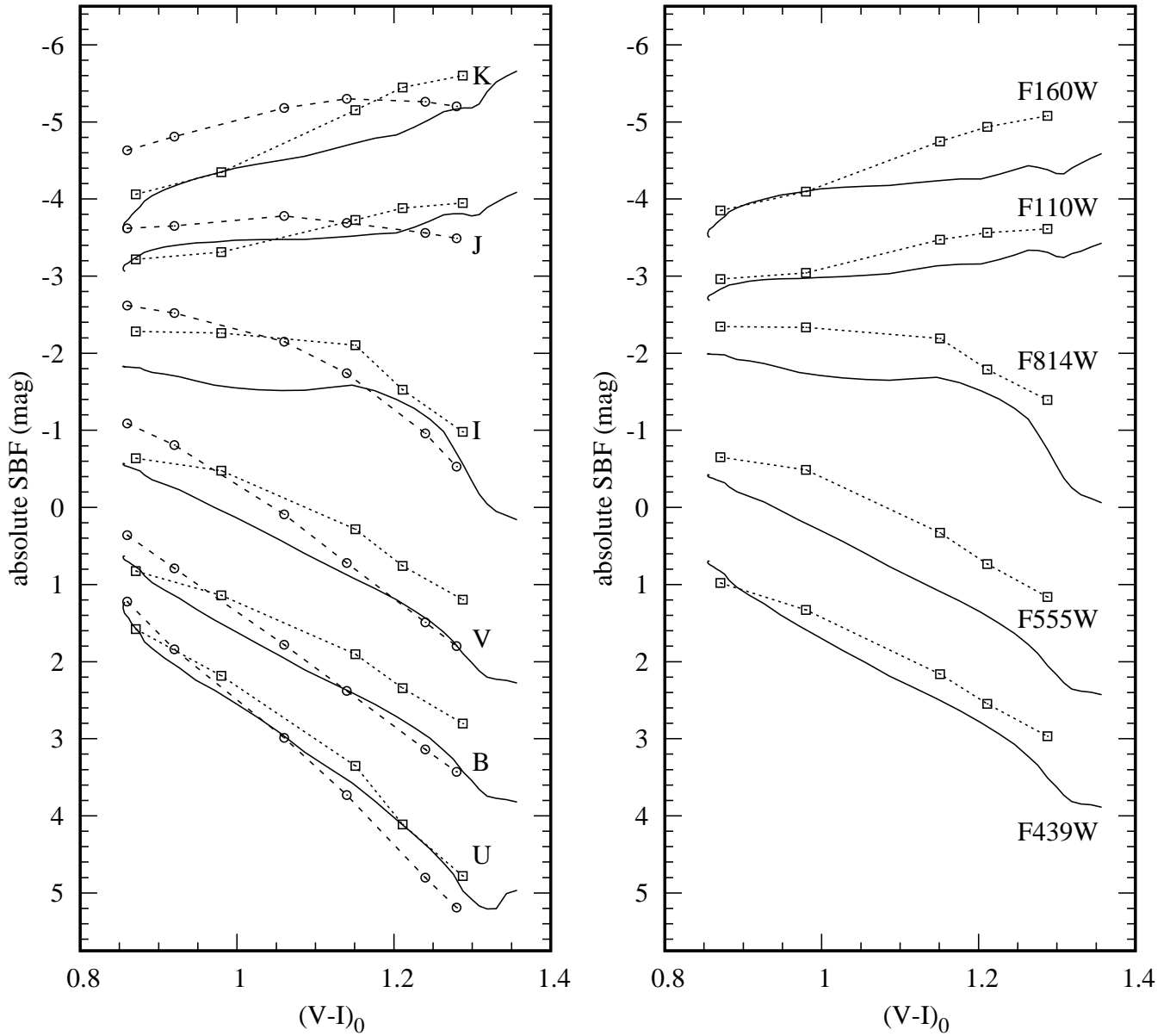
Figure 9. Comparison of the YEPS model with Blakeslee et al. (2001) and Cantiello et al. (2003) models. ( Left panel ) The absolute SBF magnitudes of SSPs in Johnson-Cousins UBVR IJK are presented. Dashed-circle, dotted-square, and solid lines are, respectively, for the SBF models from Blakeslee et al. (2001), Cantiello et al. (2003), and YEPS. To compare similar-age SBFs, the ages of SBF models from Blakeslee et al. (2001) and Cantiello et al. (2003) are, respectively, chosen as 12.6 and 13 Gyr, which are equivalent to 12 Gyr of YEPS (Chung et al. 2013a). The initial He abundance for all models is Y_{\text{ini}} = 0.23 . All models assume the standard Salpeter index for the slope of the IMF. The SBF magnitudes and the integrated (V - I)_0 color are given in the Vega mag system. Our models are placed in the lower parts of the other two models. ( Right panel ) The same as the left panel but for the selected HST filters.
