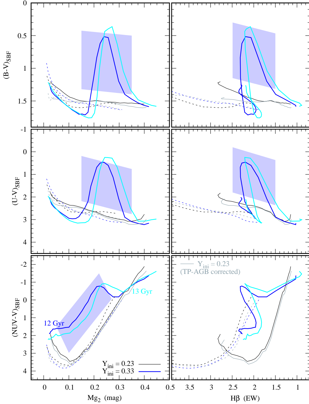
Figure 14. Theoretical predictions for SBF colors as functions of absorption-line strengths. The SBF colors of (B - V)_{\text{SBF}} , (U - V)_{\text{SBF}} , and (NUV - V)_{\text{SBF}} are presented from top to bottom panels as functions of Mg_2 (left column) and H\beta (right). Black and blue lines are the models for Y_{\text{ini}} = 0.23 and 0.33 , respectively. Dashed and solid lines are the models for 3 and 12 Gyr, respectively. Gray lines indicate models for Y_{\text{ini}} = 0.23 after the TP-AGB correction. Cyan lines are the 13 Gyr models for Y_{\text{ini}} = 0.33 , showing how older-age and He-rich models behave. The SBF colors are derived from SBF magnitudes based on the Vega mag system. Light blue boxes indicate the regions where old, He-rich populations are expected to occupy exclusively.
