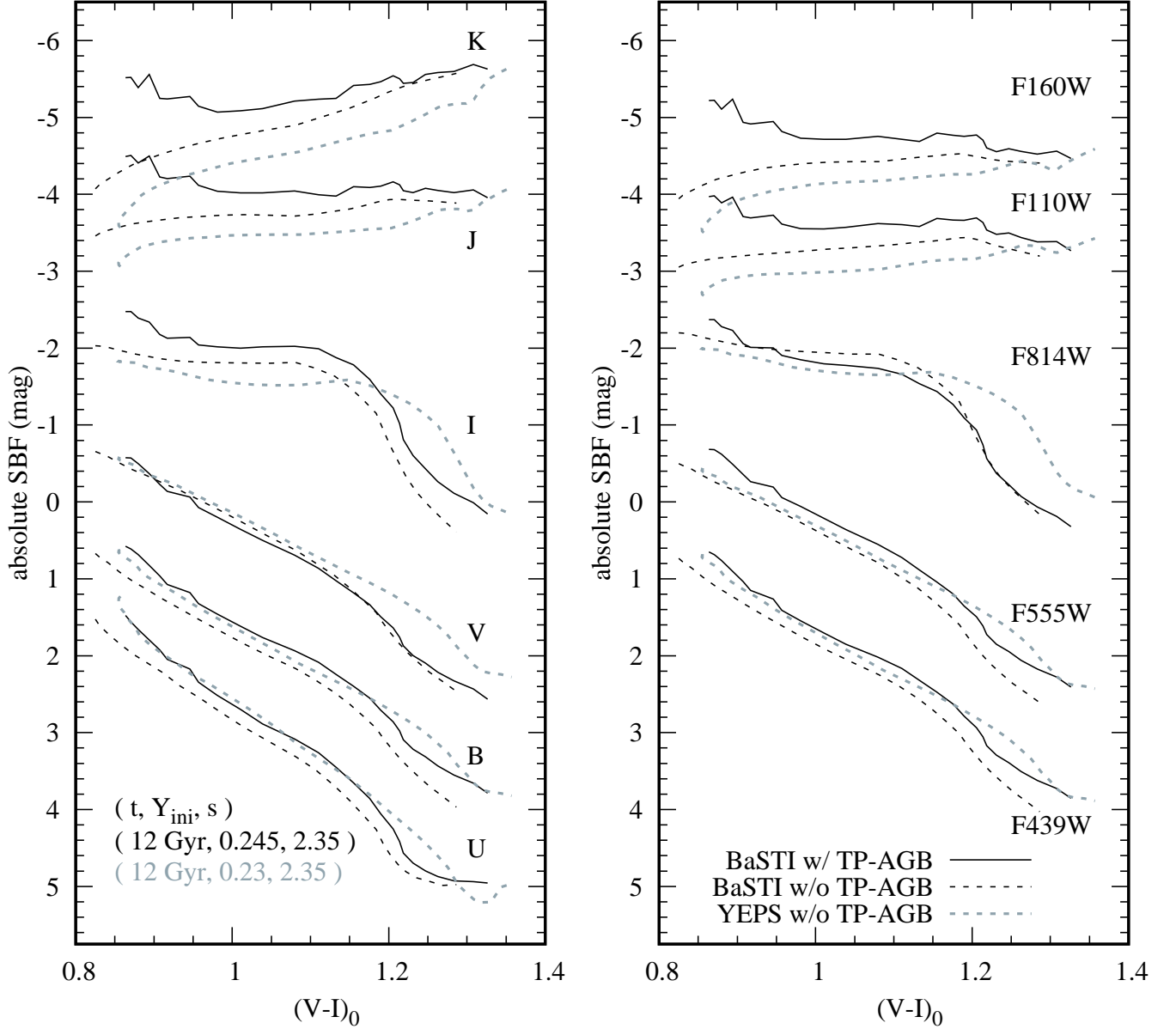
Figure 8. Comparison in the SBF versus (V-I)_0 planes among the models using the BaSTI isochrones with TP-AGB stars (black solid lines) and without them (black dashed lines), and the canonical YEPS model (gray dashed lines). All SBF magnitudes are given in the Vega mag system, and the integrated (V-I)_0 color is based on the Vega mag system. ( Left panel ) The same as the left panel of Figure 7, but with the x-axis of (V-I)_0 instead of [\text{Fe}/\text{H}] . The adopted parameters for each model are denoted in the parenthesis at the bottom. ( Right panel ) The same models for the selected HST filters.
