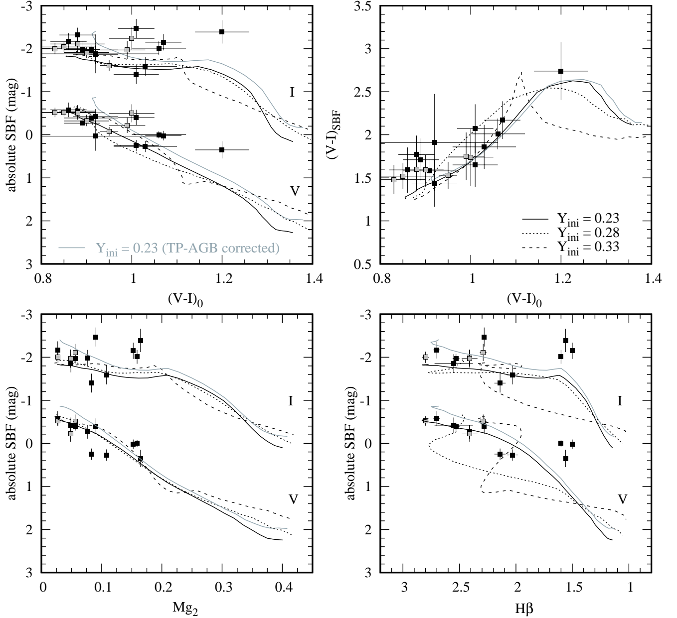
Figure 10. Comparisons between the YEPS SBF model and Galactic GC observations. The upper row shows the absolute V - and I -SBF magnitudes (upper-left panel) and (V - I)_{\text{SBF}} (upper-right) as functions of (V - I)_0 . The lower row shows the absolute V - and I -SBF magnitudes as a function of Mg_2 (lower-left) and H\beta (lower-right). The absorption indices of Galactic GCs are obtained from Kim et al. (2016). Different initial He assumptions of Y_{\text{ini}} = 0.23, 0.28, and 0.33 are, respectively, shown as solid, dotted, and dashed lines. The model parameters for age and the slope of the IMF are, respectively, 12 Gyr and s = 2.35 . All SBF magnitudes and the integrated (V - I)_0 color are given in the Vega mag system. The same Y_{\text{ini}} = 0.23 models after applying the TP-AGB correction are shown in gray lines. Squares are the SBFs of Galactic GCs from Ajhar & Tonry (1994). Gray squares mark Galactic GCs hosting extreme HB stars classified by Lee et al. (2007).
