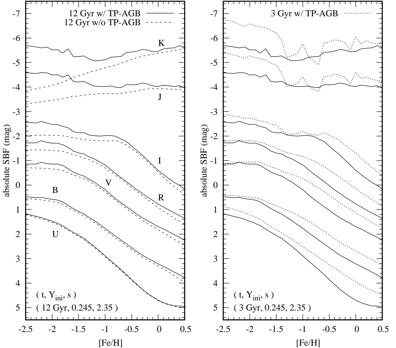
Figure 7. SBF models with and without inclusion of TP-AGB stars. The employed stellar evolution tracks for this model are the BaSTI isochrones (Pietrinferni et al. 2006). All SBF magnitudes are given in the Vega mag system. The adopted stellar parameters for the model are denoted in the parenthesis at the bottom of each panel. ( Left panel ) Solid and dashed lines are the SBF models with and without TP-AGB stars, respectively. ( Right panel ) Dotted and solid lines are, respectively, 3 and 12 Gyr models with TP-AGB stars for the same passbands as the left panel.
