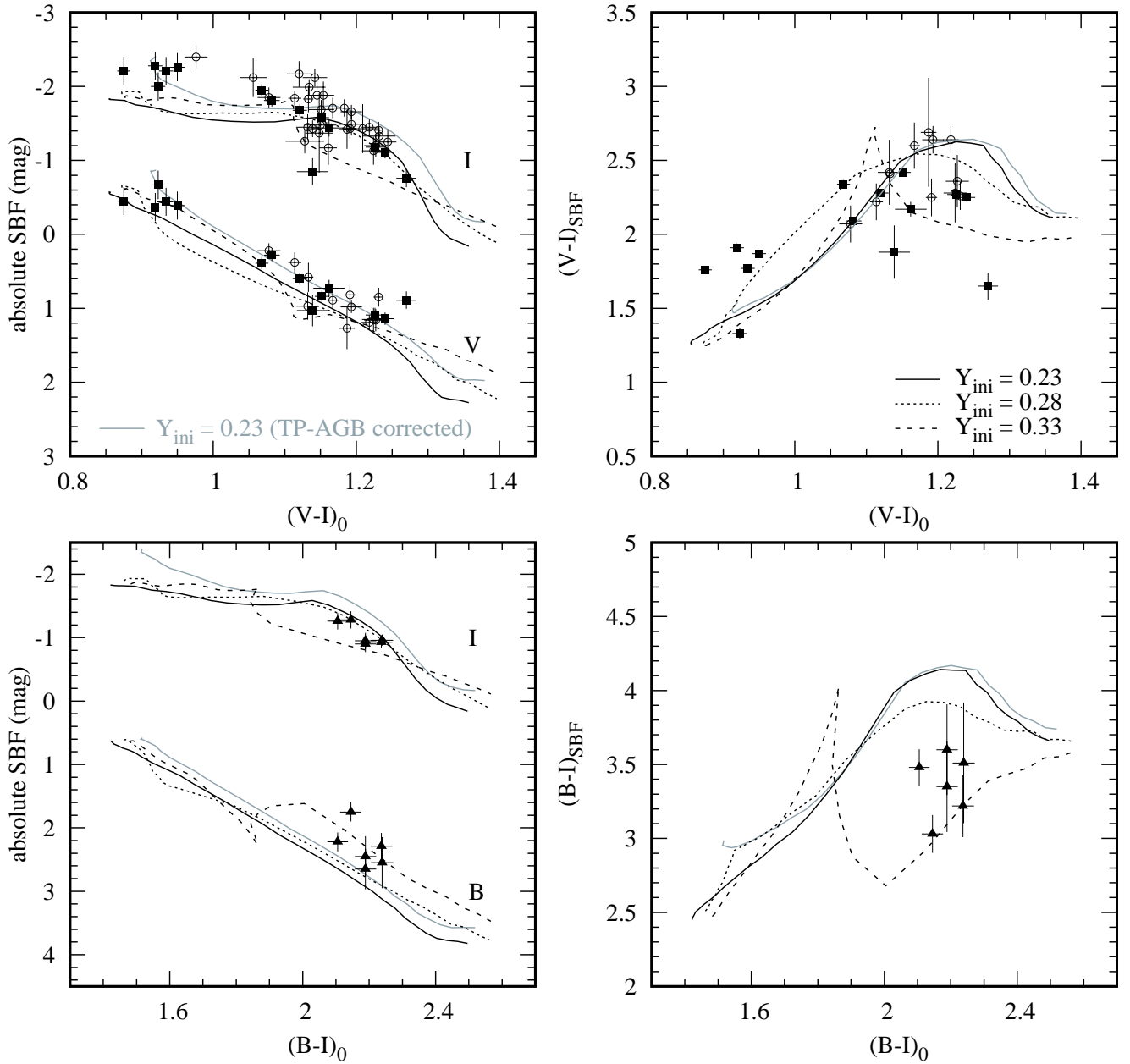
Figure 11. ( Upper panels ) Comparisons between the YEPS SBF model and early-type galaxy observations in V and I . The absolute V - and I -SBF magnitudes (left panel) and (V - I)_{\text{SBF}} (right) are shown as functions of (V - I)_0 . The SBF models are the same as in Figure 10. Filled squares are early-type galaxies from the HST ACS observation by Cantiello et al. (2007b). Open circles are early-type galaxies from data compiled by Cantiello et al. (2003). ( Lower panels ) Same as the upper panels but for B and I SBFs. Filled triangles are six early-type galaxies from the HST ACS observation by Cantiello et al. (2007a).
