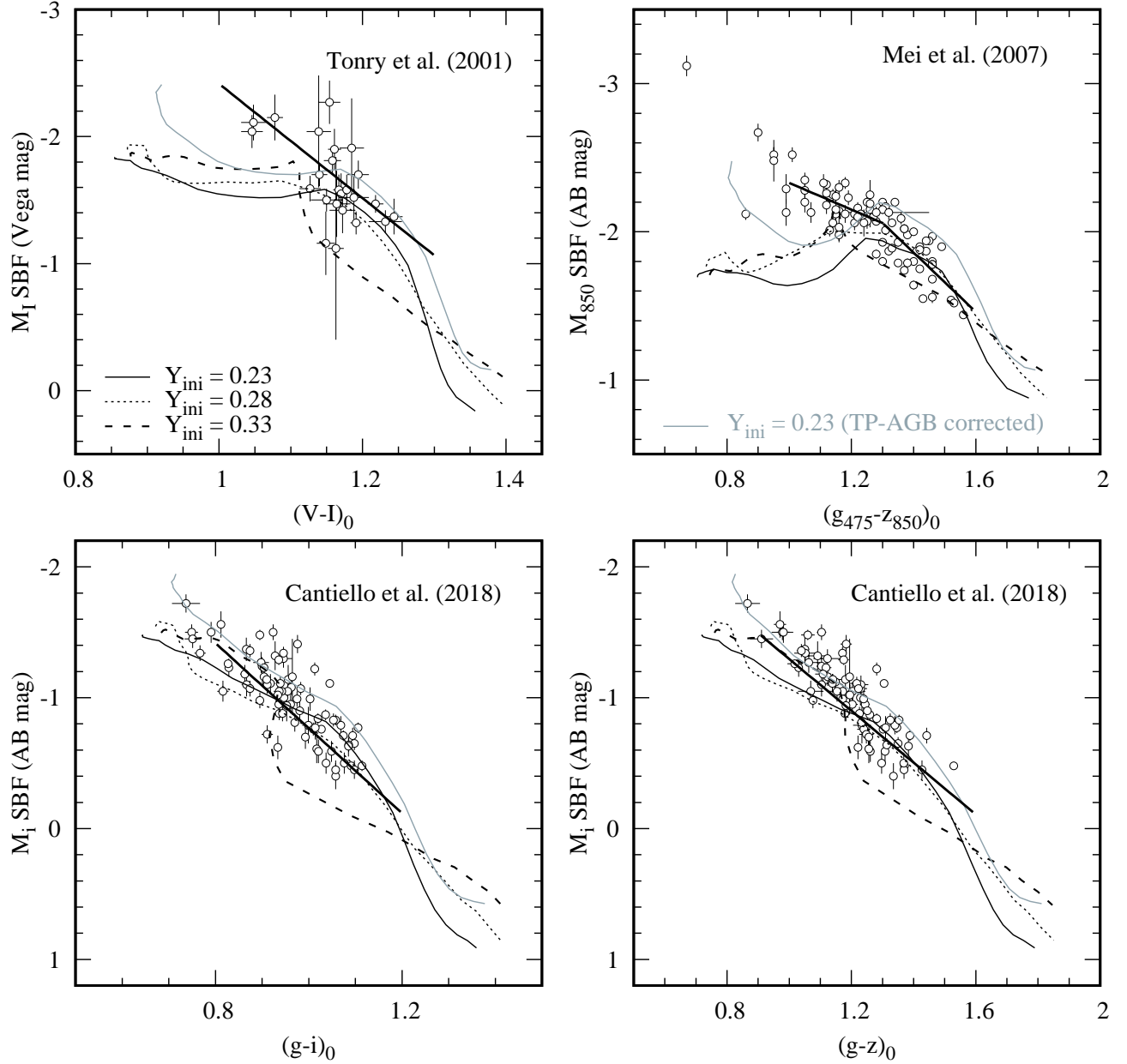
Figure 12. Comparing the empirical SBF versus color relations with the YEPS SBF predictions. Open circles are early-type galaxies in the Virgo Cluster and data are from Tonry et al. (2001) , Mei et al. (2007) , and Cantiello et al. (2018) . Thick solid lines are empirical SBF–color relations in the literature. Solid, dotted, and dashed lines are for different assumptions on the initial He of Y_{\text{ini}} = 0.23 , 0.28 , and 0.33 . The SBF models for z_{850} - and i -bands are in the AB mag system, and the integrated colors for those bands follow the same photometric system. The same Y_{\text{ini}} = 0.23 models after applying the TP-AGB correction are shown in gray lines. The adopted distance modulus for the Virgo Cluster is (m - M)_{\text{Virgo}} = 31.09 mag ( Blakeslee et al. 2009 ).
