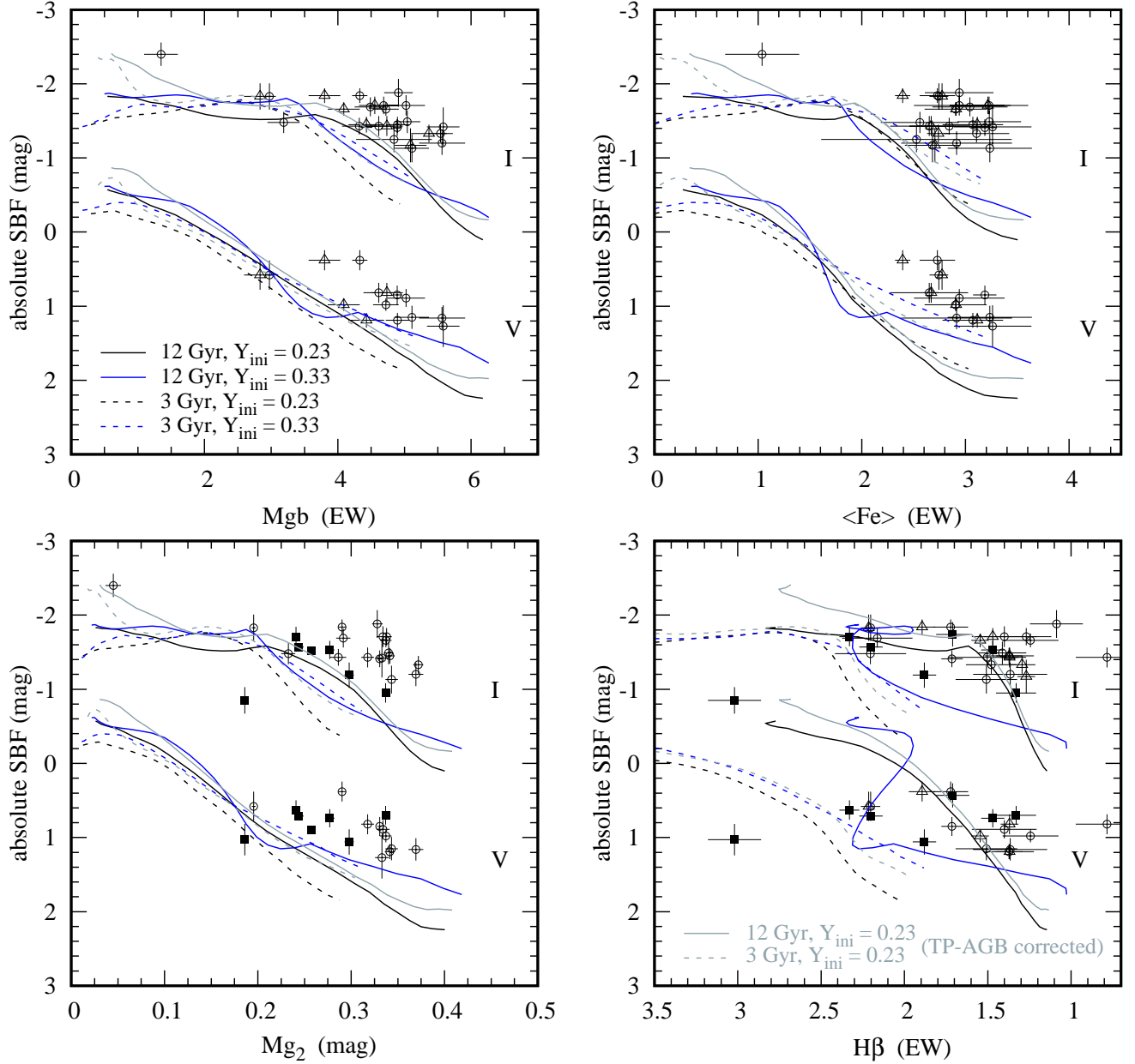
Figure 13. Comparisons between the YEPS SBF model and early-type galaxy observations in the absolute SBF mags versus absorption indices planes. The absolute V - and I -SBF mags are shown as functions of Mgb (upper-left panel), \langle Fe \rangle (upper-right), Mg_2 (lower-left), and H\beta (lower-right). Black and blue solid (dashed) lines are the 12 Gyr (3 Gyr) models for Y_{ini} = 0.23 and 0.33, respectively. Gray solid (dashed) lines are 12 Gyr (3 Gyr) models for Y_{ini} = 0.23 after applying the TP-AGB correction. The slope of the IMF is s = 2.35 for all models. All SBF magnitudes are in the Vega mag system. Open symbols are galaxies which have the SBF data from Cantiello et al. (2003) and the absorption-line data from Lee & Worthey (2005) (circles) and Sánchez-Blázquez et al. (2006) (triangles). Filled squares in the lower panels are galaxies with the SBF data from Cantiello et al. (2007a) .
